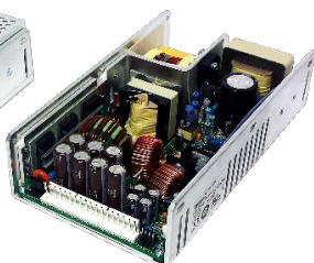
OPEN CHASSIS
