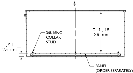
SECTION X-X
