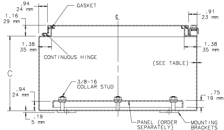
SECTION X-X
