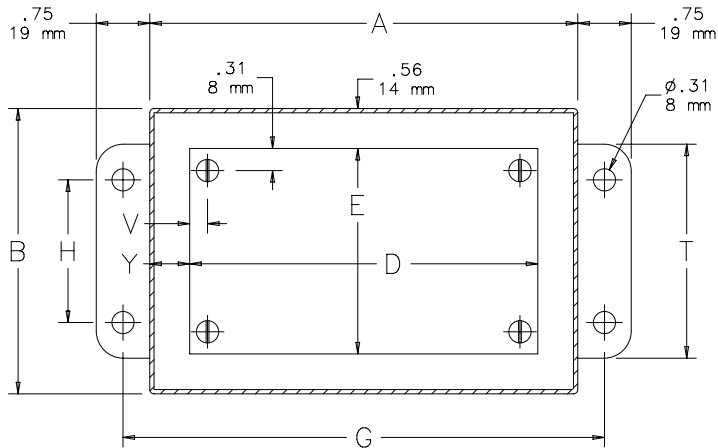
SECTION Y-Y
