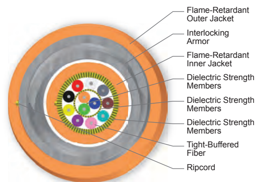
Cross Section of Part Number: 012K88-33130-A3
