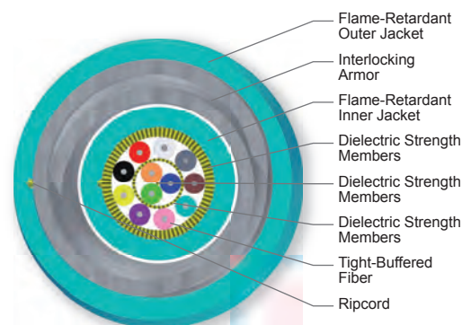
Cross Section of Part Number: 012T81-33190-A1
