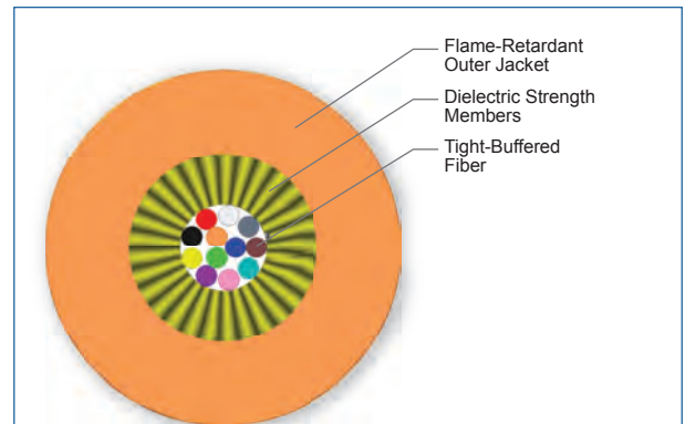
Cross Section of Part Number: 012TD8-31331-20
