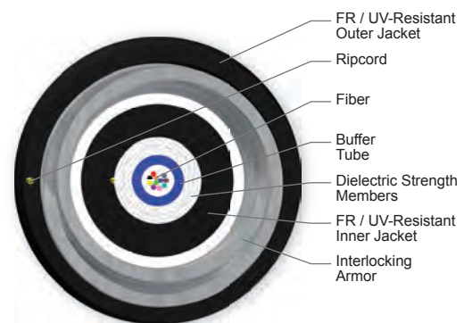
Cross Section of Part Number: 012TSF-T4131DA1
