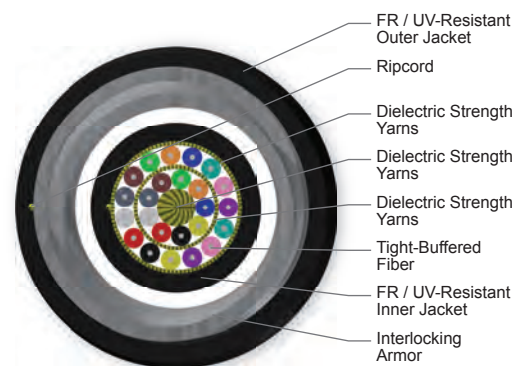
Cross Section of Part Number: 024E8F-31131-A1
