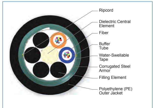
Cross Section of Part Number: 024EUC-T4100D20
