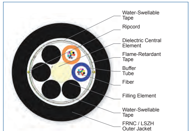
Cross Section of Part Number: 024KUZ-T4130D2N
