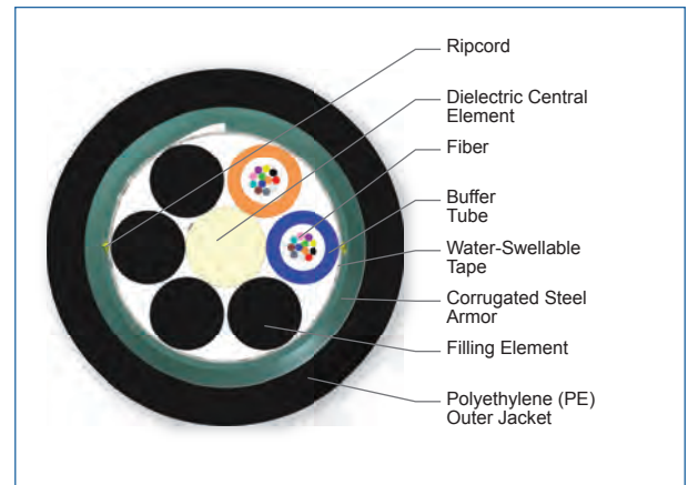
Cross Section of Part Number: 024TUC-T4180D20
