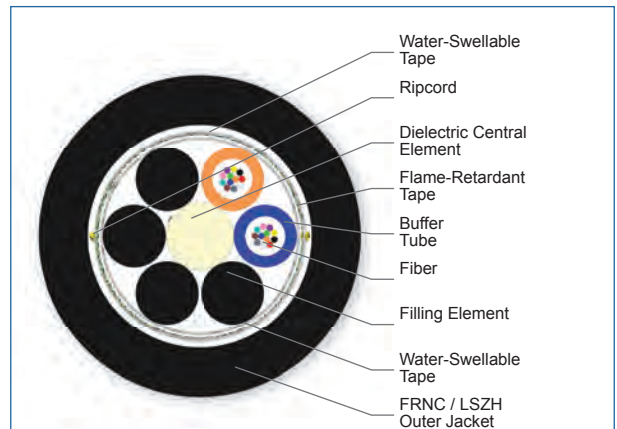
Cross Section of Part Number: 012EUZ-T4101D2N
