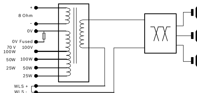
Circuit diagram
