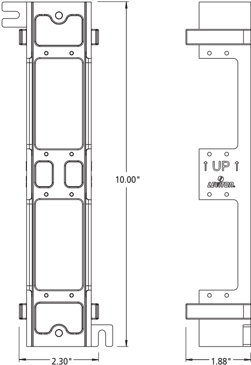
89D Mounting Bracket (Available separately)
