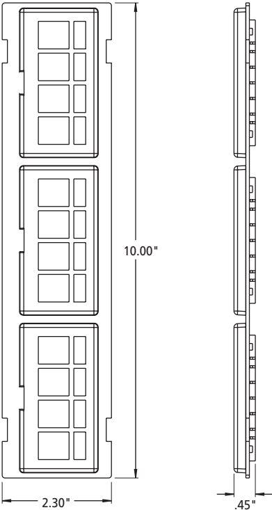
QuickPort 12-Port Patch Block
