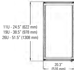
Front View (Gate Closed)
