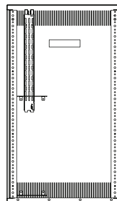
OPTIONAL LEVERLOCK INSIDE VIEW
