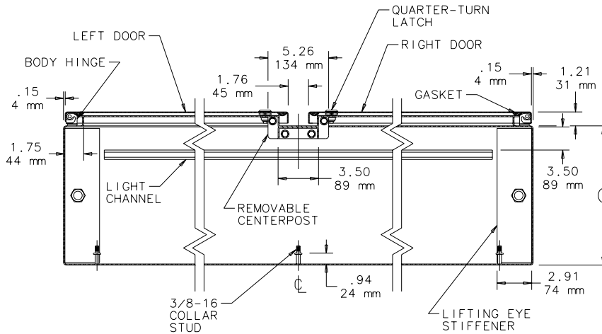
SECTION X-X
