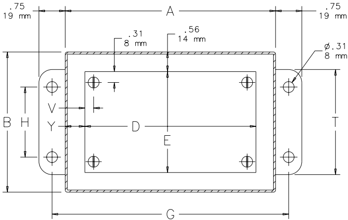
SECTION Y-Y
