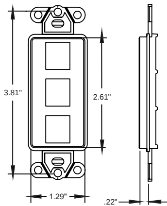
3-Port Insert
