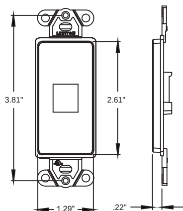
1-Port Insert
