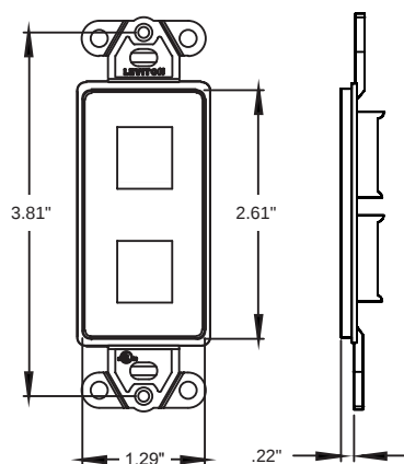
2-Port Insert
