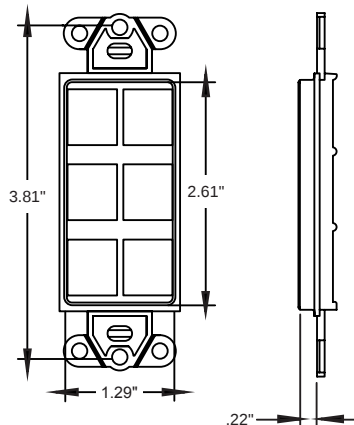
6-Port Insert
