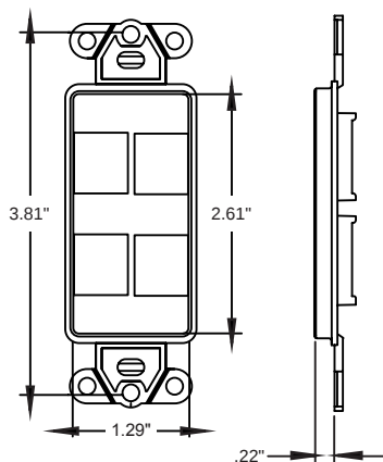
4-Port Insert
