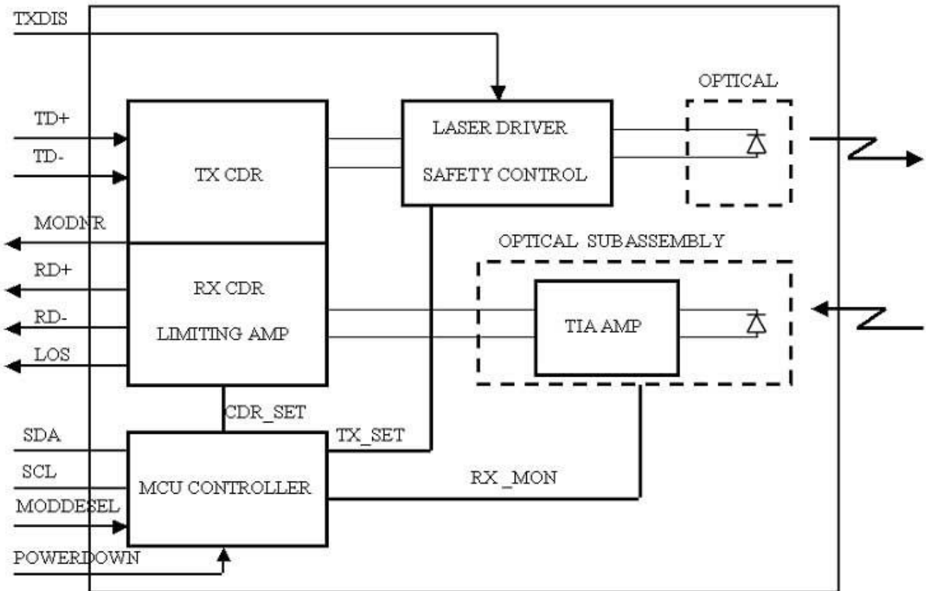
Block Diagram
