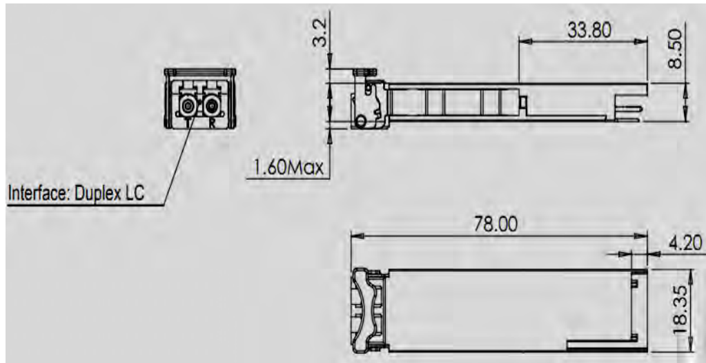
Figure 5. Mechanical Outline
