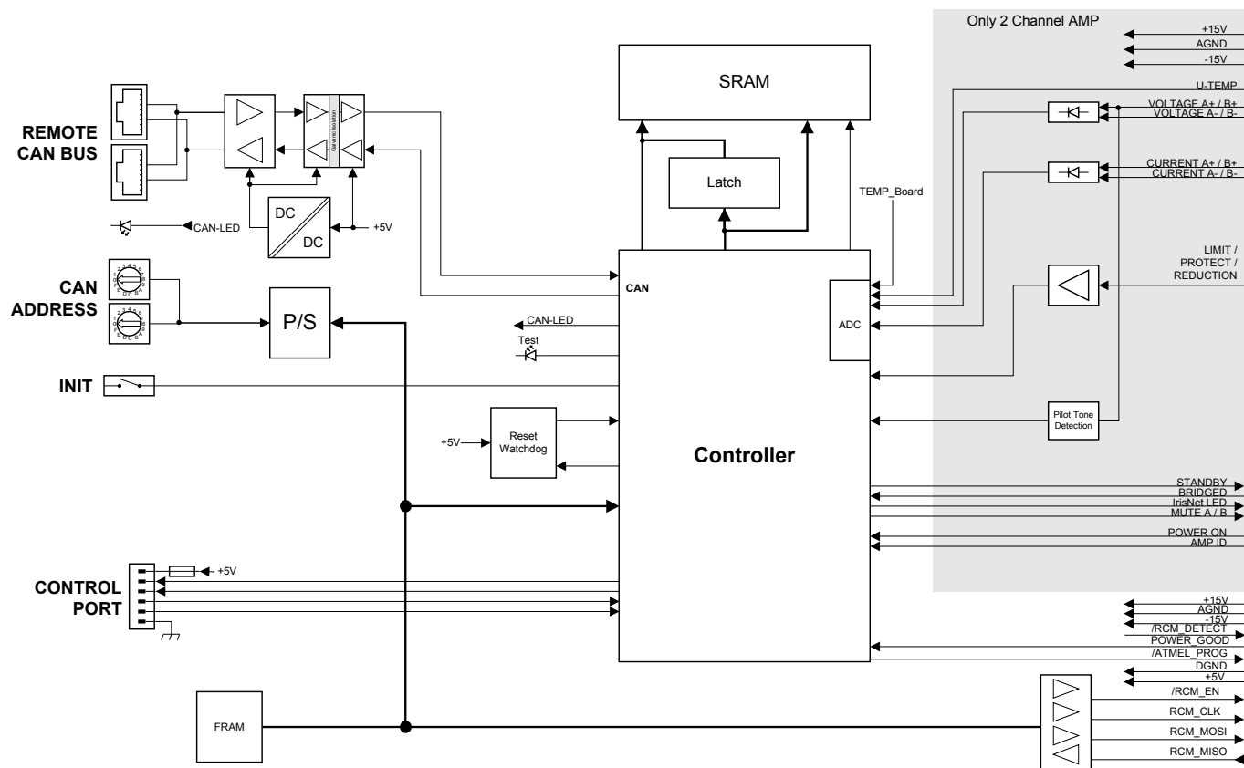
Circuit diagram
