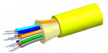
760018515 | R-024-DS-8W-FSUYL Riser Distribution Cable, 24 fiber single-unit
