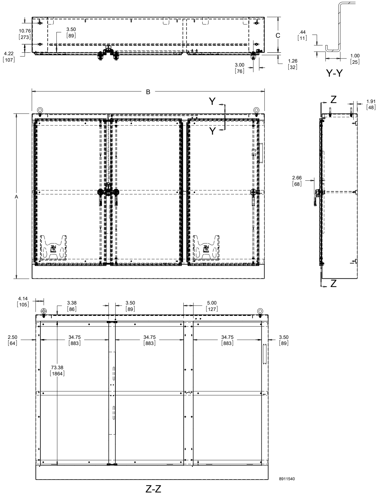
THREE-DOOR ENCLOSURE
