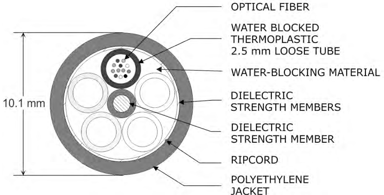
Cross-section Diagram - LTD12B012-M2
