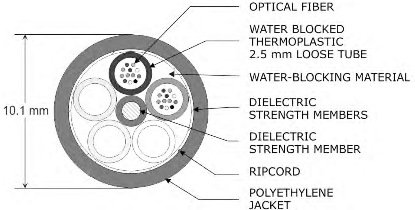
Cross-section Diagram - LTD12B024-M2
