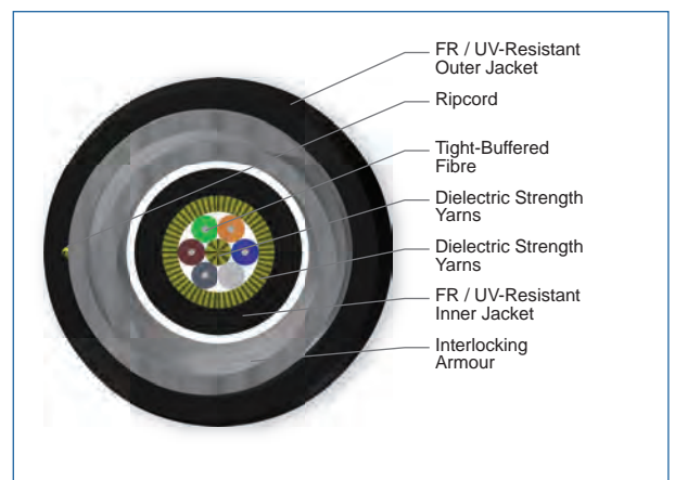
Cross Section of Order Number: 006E8P-31131-A3
