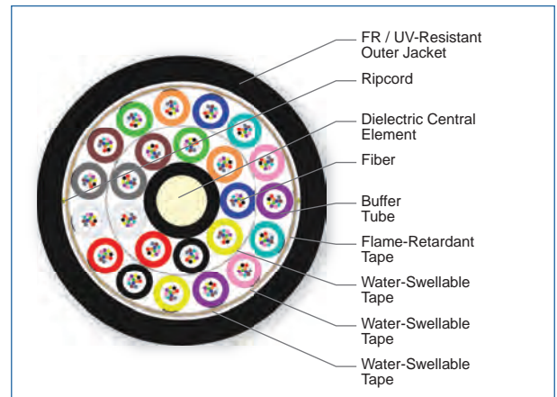
Cross Section of Part Number: 288EUF-T4101D20
