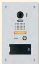
JP-DVF-RP10* Card Access Video Door Station • HID® multiCLASS SE® Proximity Card Reader • PTZ camera • Stainless steel panel • Weather and vandal resistant • Flush mount (back box included)
