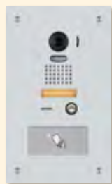
JP-DVF-HID* Card Access Video Door Station • HID® ProxPoint® Plus Proximity Card Reader • PTZ camera • Stainless steel panel • Weather and vandal resistant • Flush mount (back box included)
