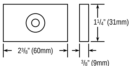
Armature Plate
