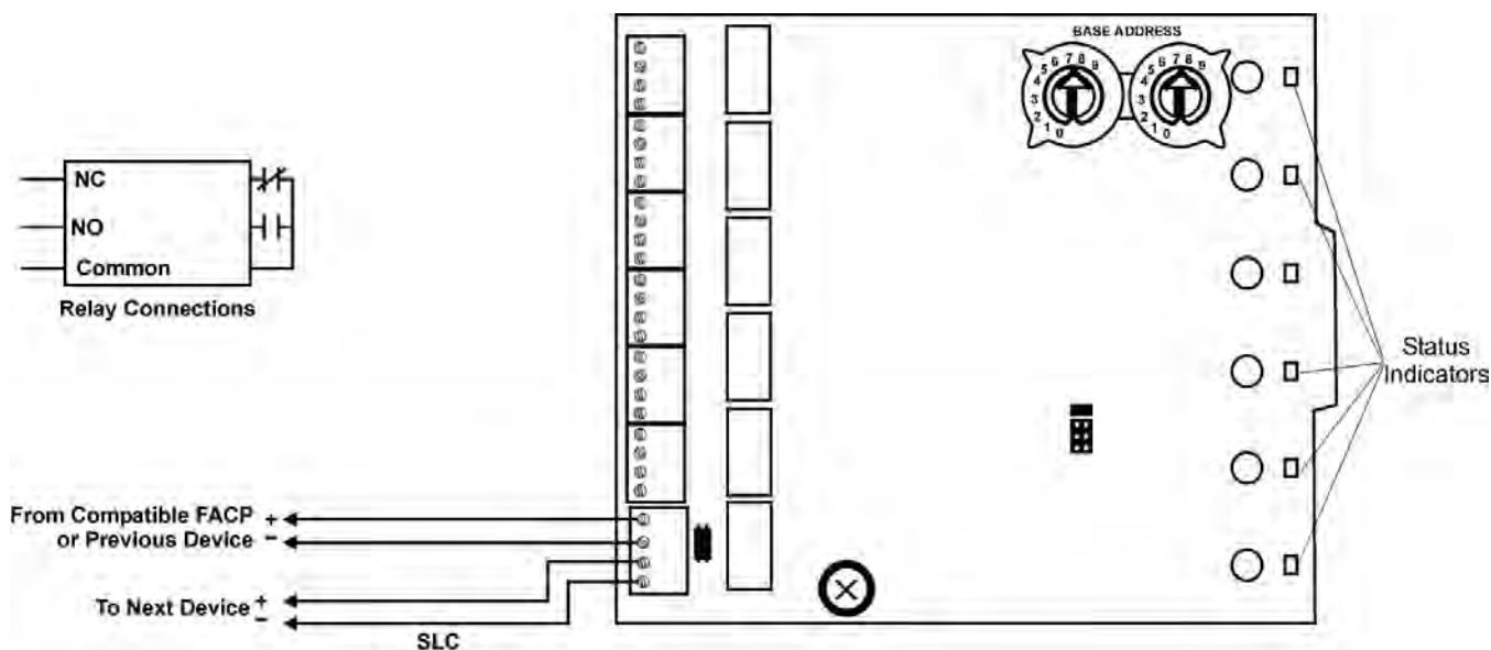
Wiring the SK-Relay-6 Relay Module
