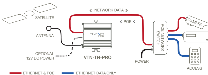
Diagram 1. TIMENET Pro delivers an accurate network time signal with maximum reliability and minimal installation effort.
