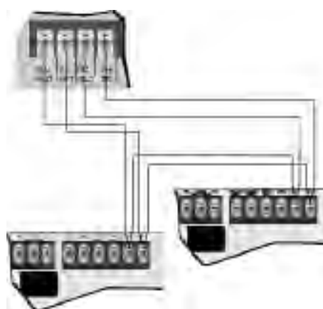
Class A (Style 6) Wiring
