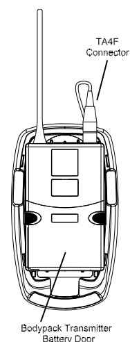
Figure 3: Bottom View with Bodypack Transmitter
