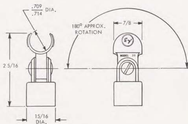
Figure 2-Dimensions-311
