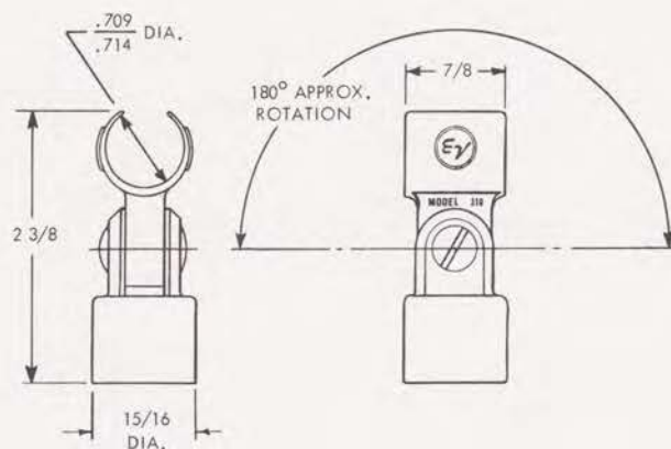
Figure 1-Dimensions-310
