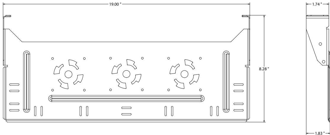
e2XHD Rear Cable Manager for flat panels
