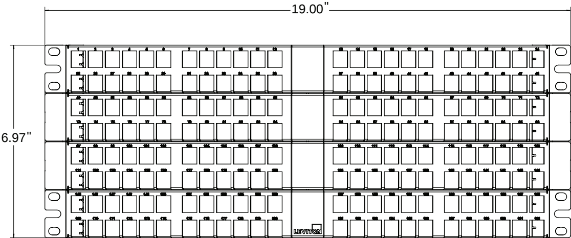
4RU Panel — Front View
