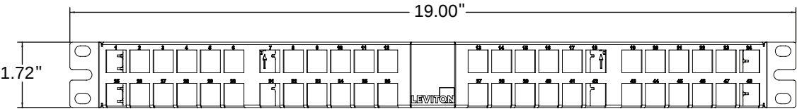
1RU Panel — Front View
