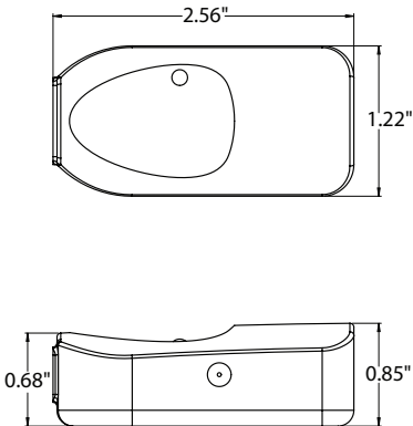
Transmitter
