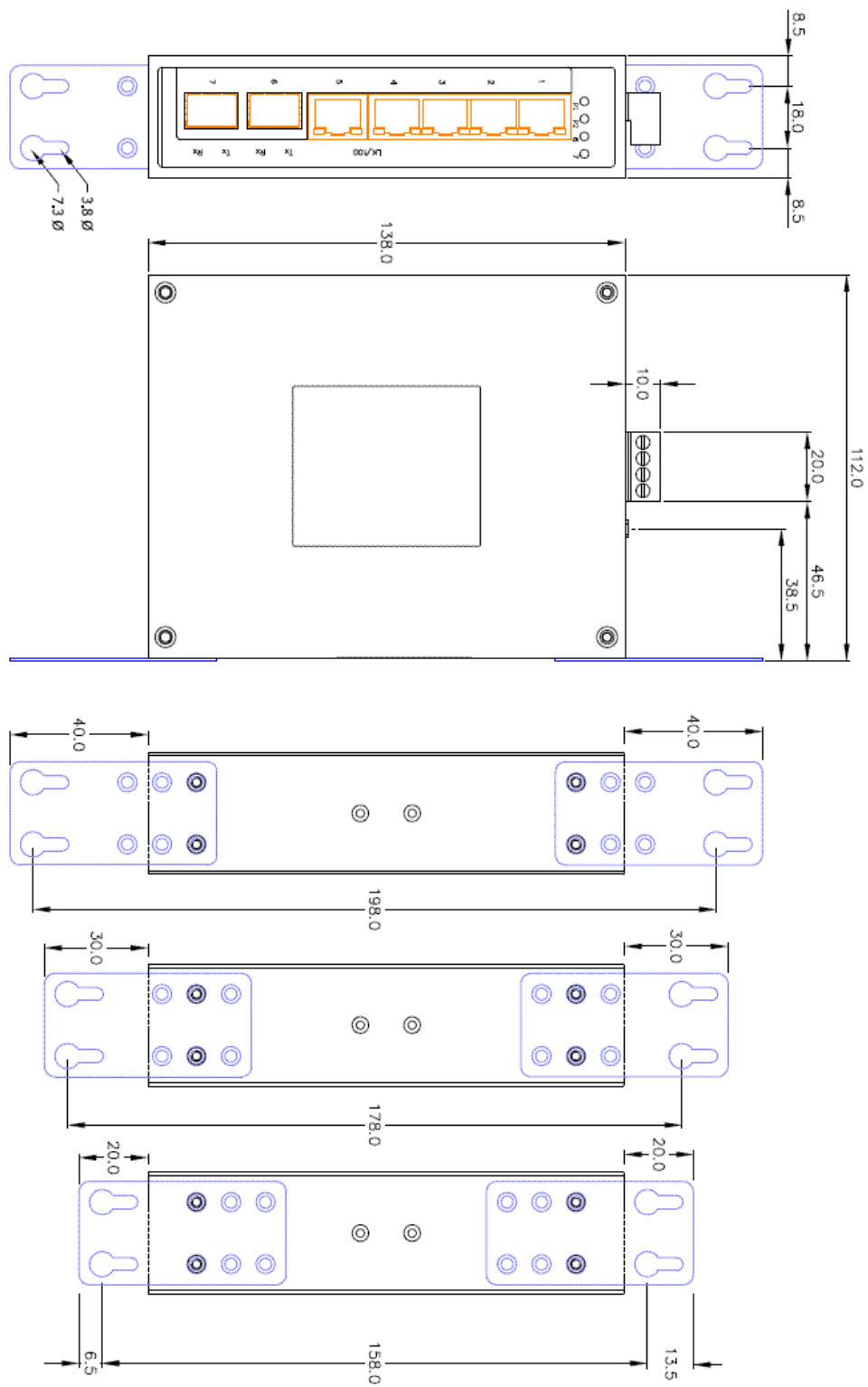
IDS-105G Industrial Gigabit Switch Diagram
