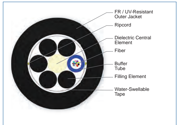
Cross Section of Part Number: 012TUF-T4180D20
