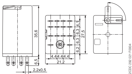
Versions with 4 c/o (SPDT) contacts (CR-M ... 4)
