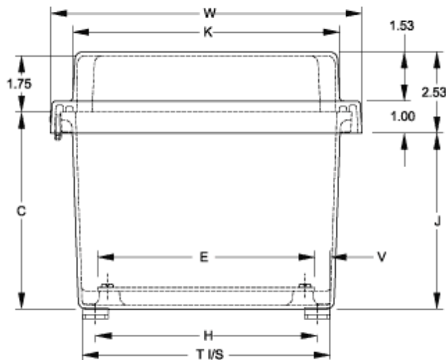
End View
