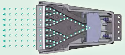
High frequencies compression driver
