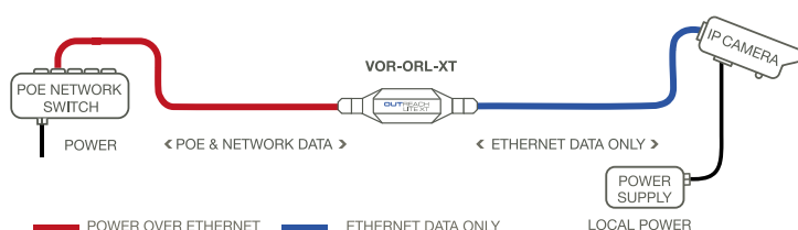
Diagram 1. OUTREACH Lite XT is powered by POE, so it can double Ethernet range without requiring local power.
