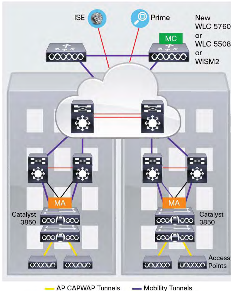
Figure 1. Mobility Controller (MC) and Mobility Agent (MA)
