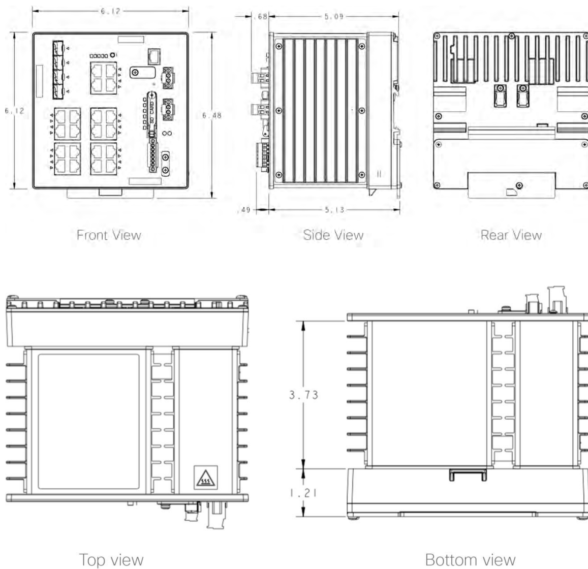
Figure 3. IE-4000 dimensions
