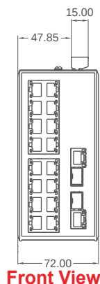
Front View
