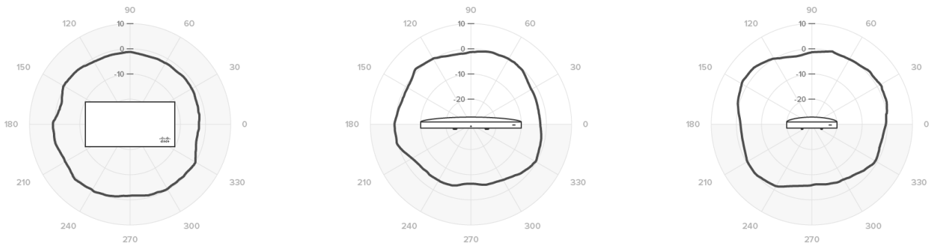
Radiation Pattern for 2.4GHz Antennas
