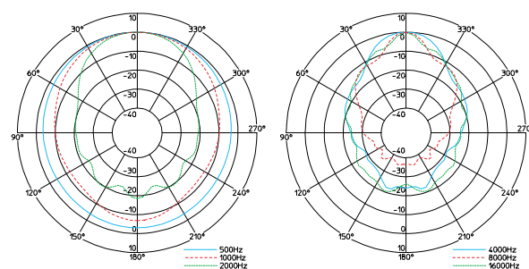
Vertical
