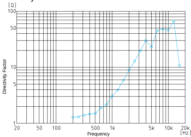
Directivity Factor
