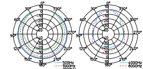
Vertical
