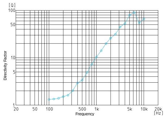
Directivity Factor
