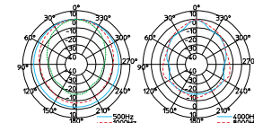
Vertical
