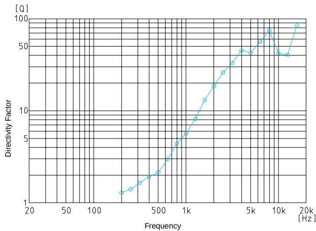
Directivity Factor
