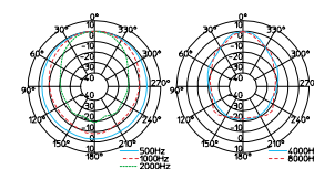
Vertical
