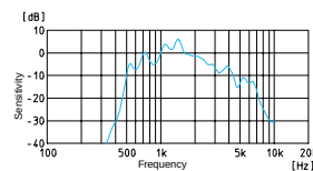
Frequency Response
