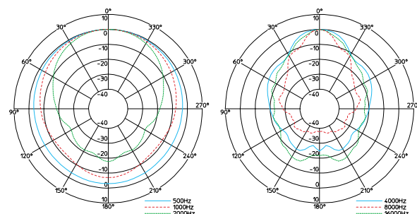
Vertical
