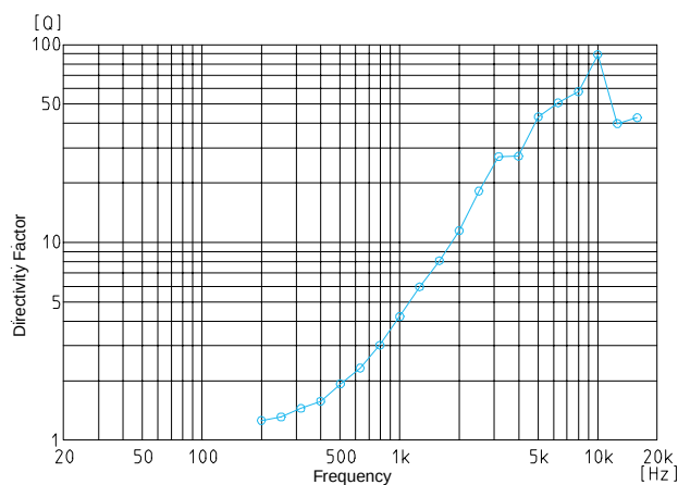
Directivity Factor
